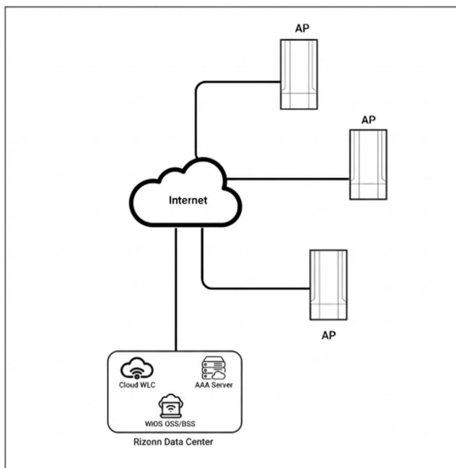
Figure 1. UniMax Access Point with Rizonn Cloud manager
